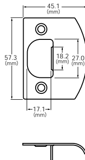
No.D203 Full-lip strike
