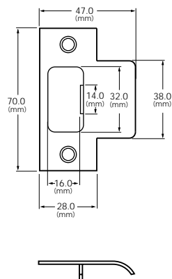
No. K203-G2 (Anti-rattle) strike
