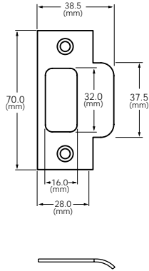
No.K203-G3 strike (standard)
