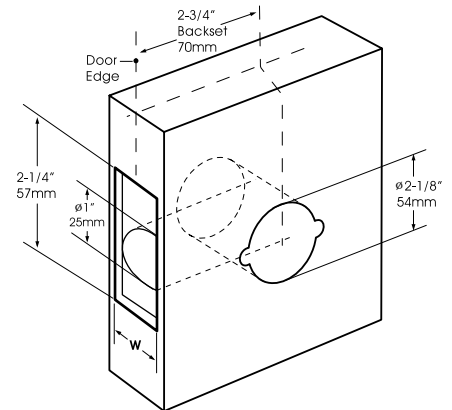
Type 4300L cutout × K203-G3 strike
