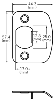
No.U203 Full-lip strike
