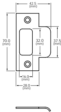
No.K203-G3 Long-lip strike
