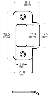
No.K203-G3 Round-corner strike
