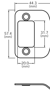
No.U204 Full-lip strike
